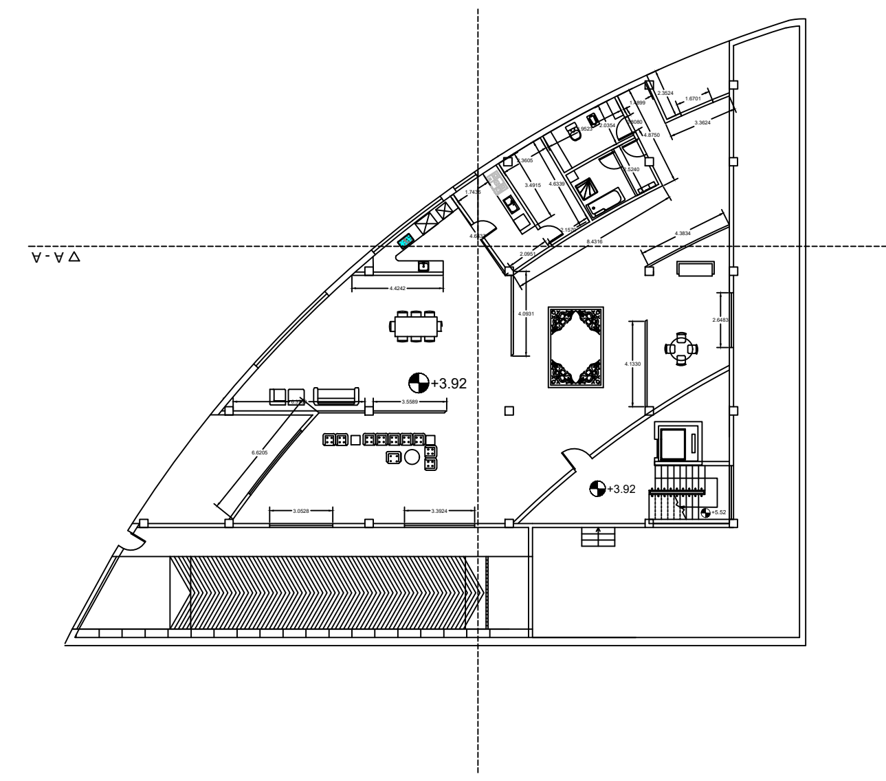
FirstFloorPlan
