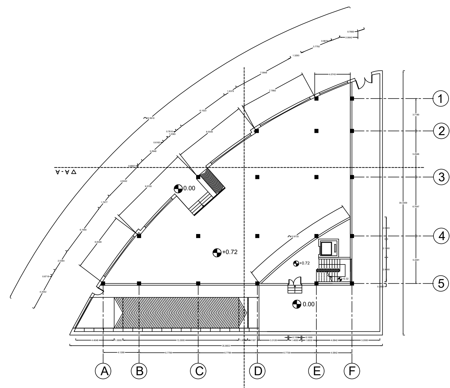
GroundFloorPlan
