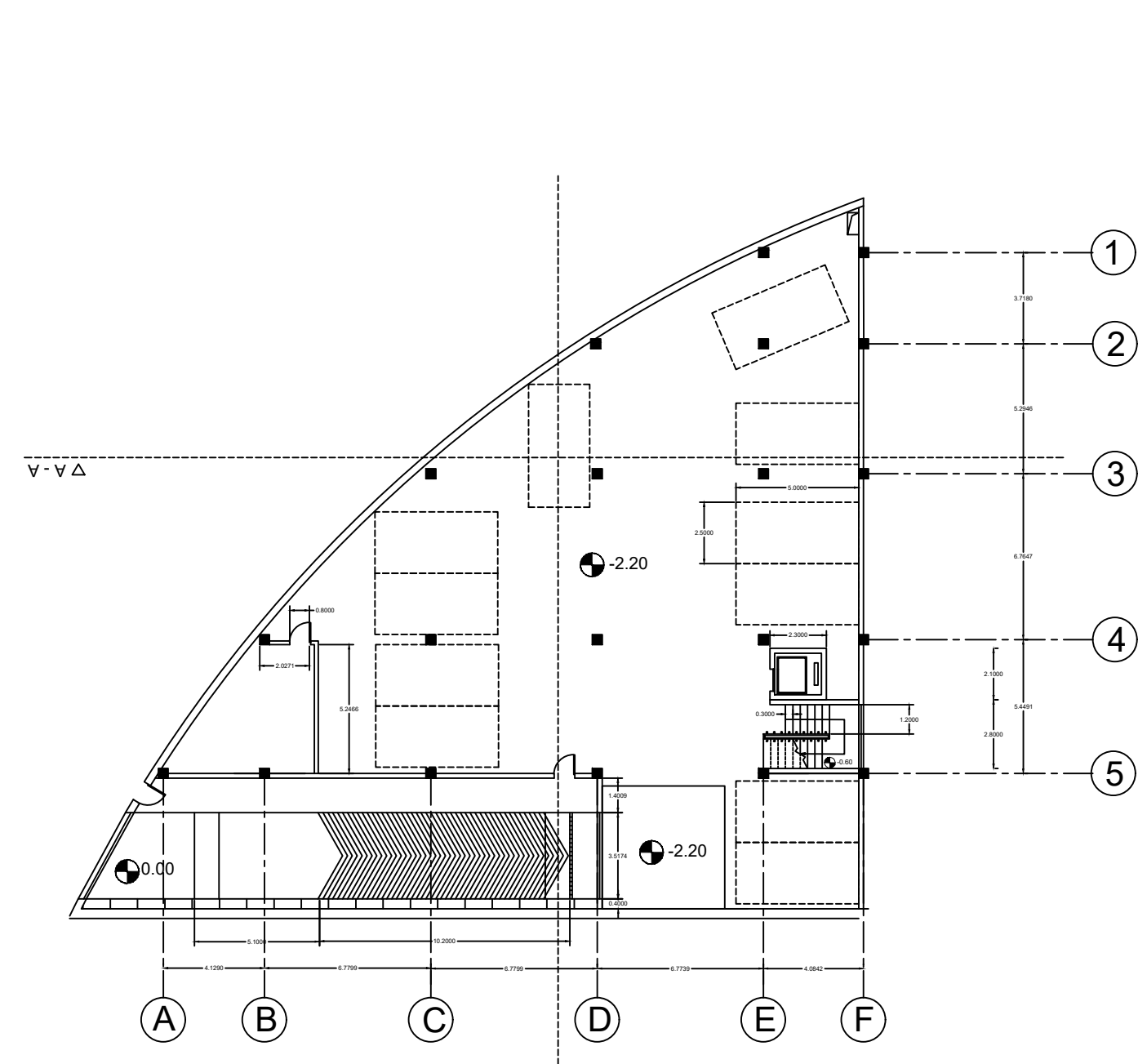
BasementPlan
