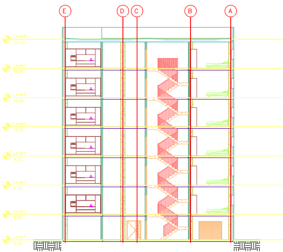
SEC A - A SC: 1/100
