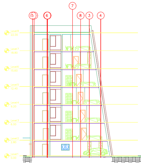
SEC B - B SC: 1/100
