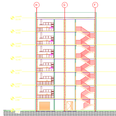
SEC C - C SC: 1/100
