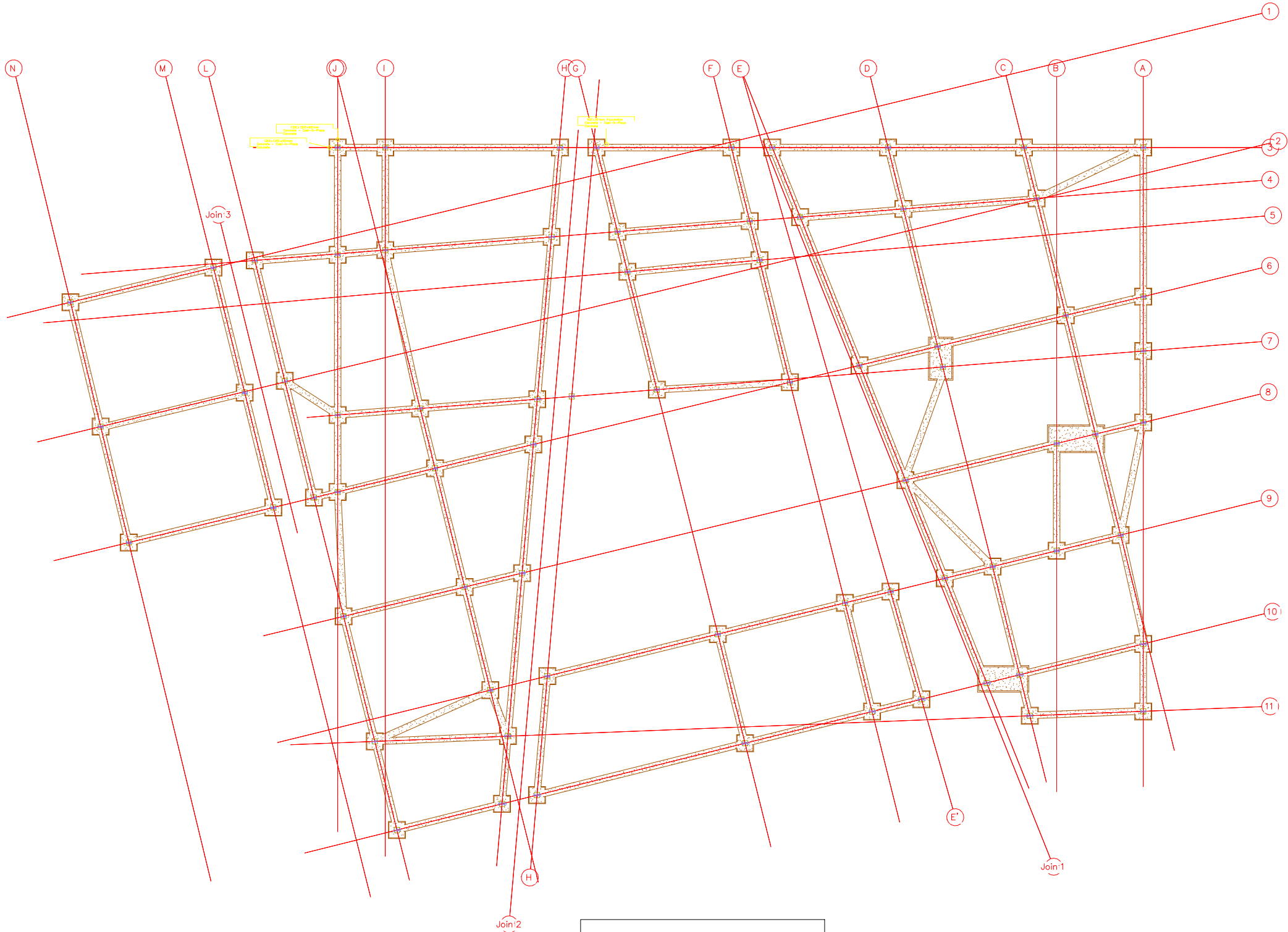
Foundation Level Sc: 1/100
